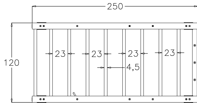
PIANTA (PLAN)
