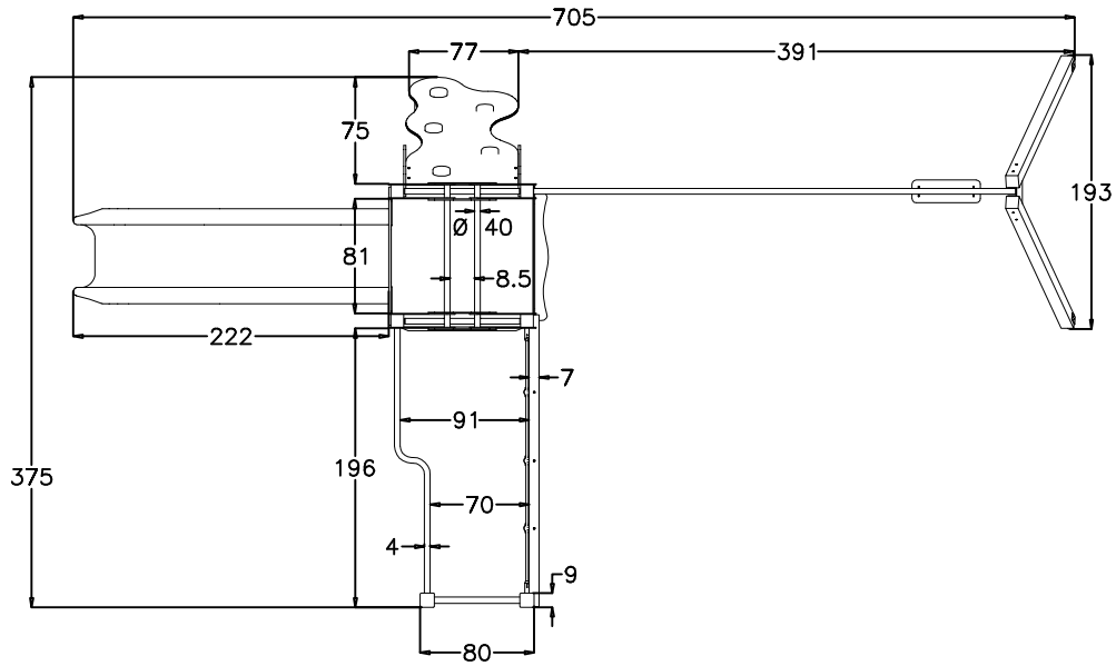
PIANTA (PLAN)
